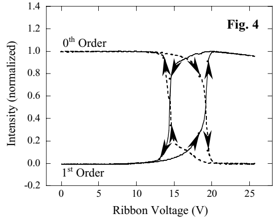
Fig. 4 Measured light intensity in the 0 th and 1 st order beams as a function of applied voltage showing hysteresis. The arrows in the bistable region indicate the permitted direction of travel.
