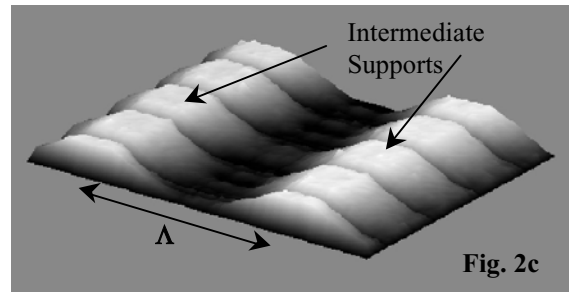
Fig. 2 Illustration of a conformal GEMS device in the actuated state (Figs. 2a and 2b) with interferometry showing the semi-conformal ribbon topography of the grating formed by a fabricated device (Figs. 2c).
