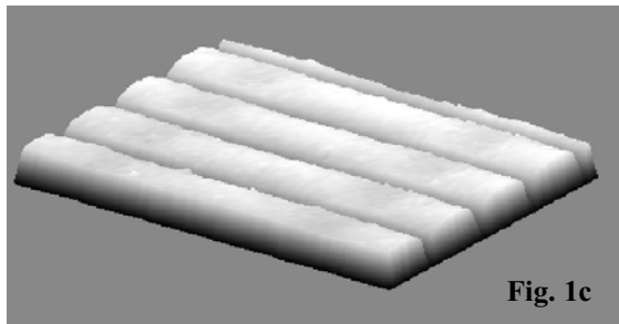
Fig. 1 Illustration of a conformal GEMS device in the unactuated state (Figs. 1a and 1b) with interferometry showing ribbon topography of a fabricated device (Fig. 1c, courtesy of Rob Gutierrez). For clarity, the vertical scale is greatly amplified relative to the horizontal.
