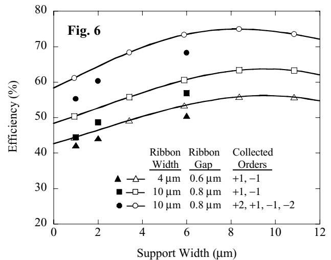
Fig. 6 Plot of device diffraction efficiency for various device designs comparing experimental results (filled markers) with theory (solid lines with open markers).
